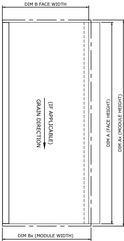
ELEVATION ON FRONT FACE OF PANEL
