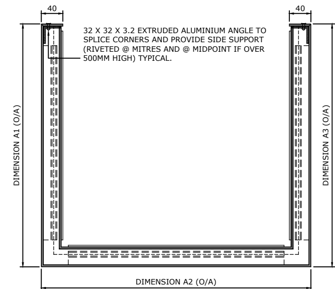
PLAN SECTION THROUGH PANEL
