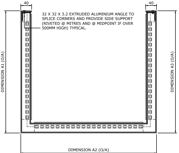
PLAN SECTION THROUGH PANEL
